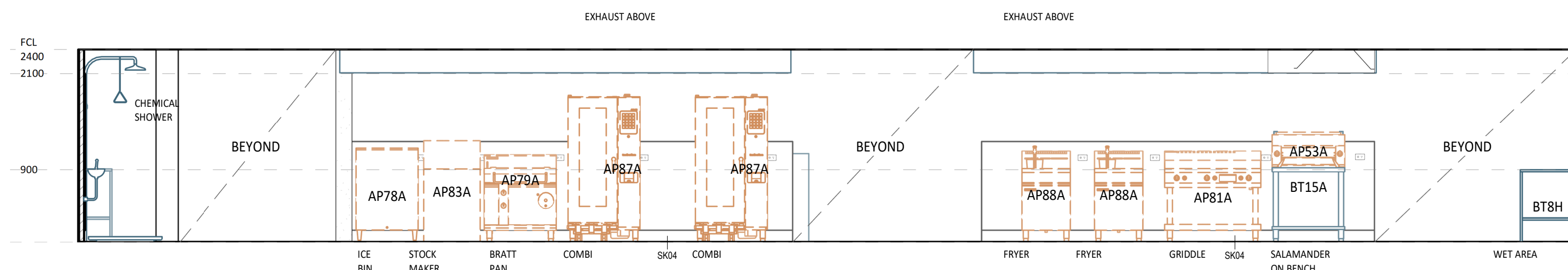
4 ELEVATION DETAIL 60-05 1 : 50
