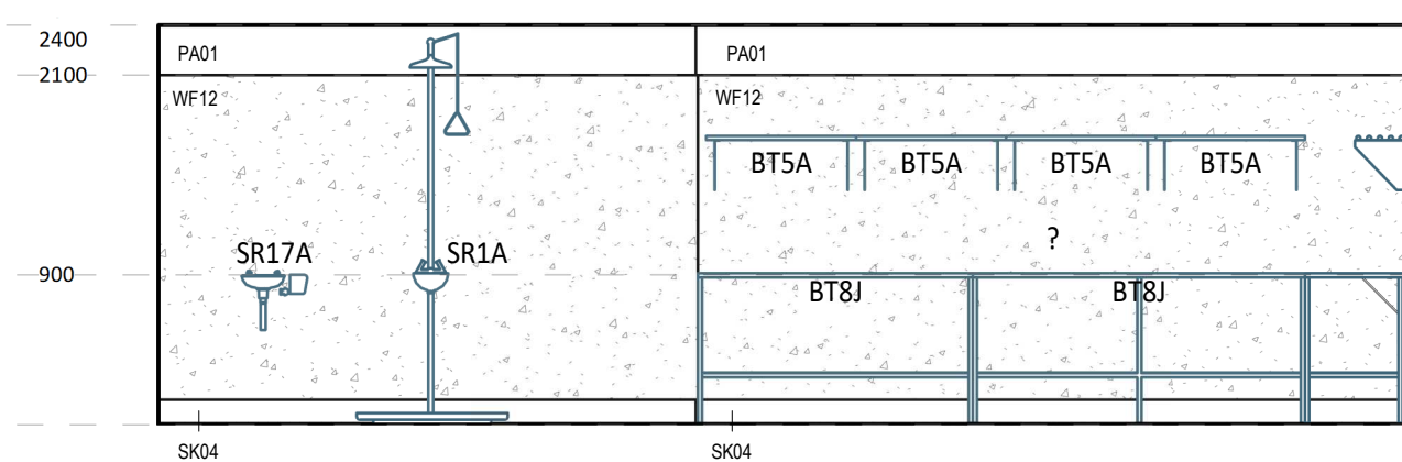
6 ELEVATION DETAIL 60-01 1 : 50
