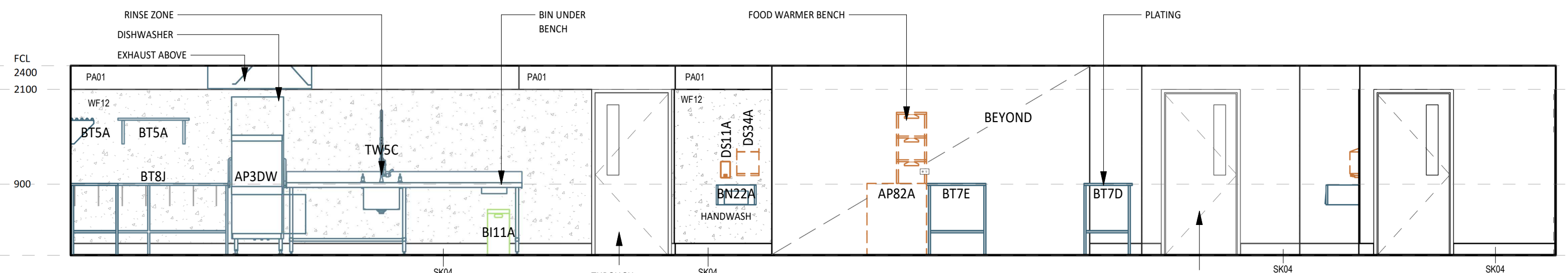
5 ELEVATION DETAIL 60-05 1 : 50
